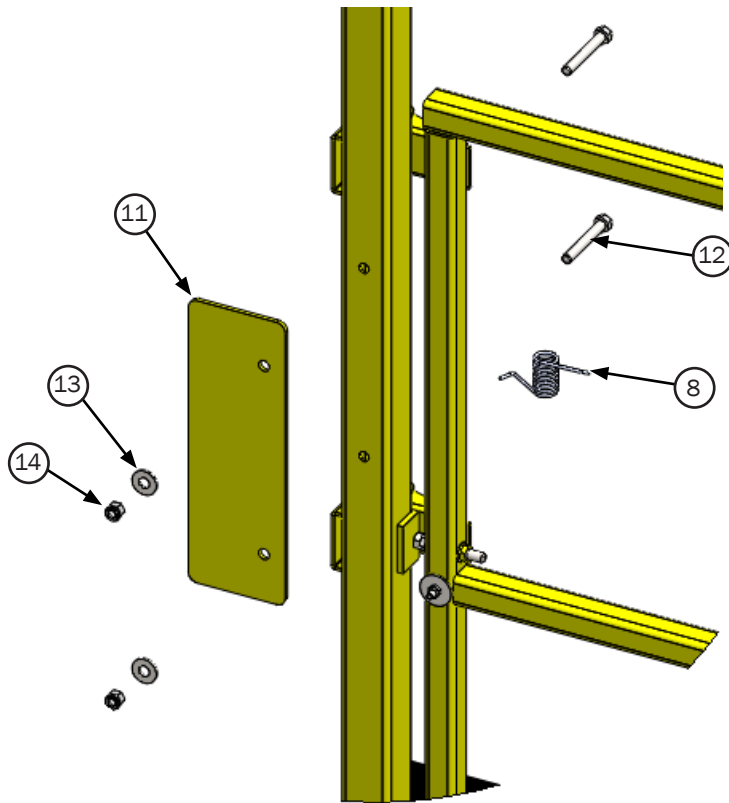
DETAIL B
