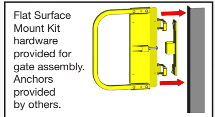
Flat Surface Mount Kit
