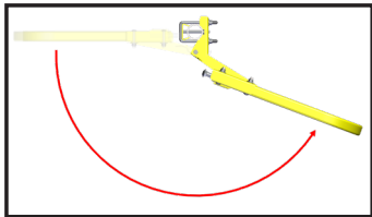
Standard Universal Hinge Bracket
