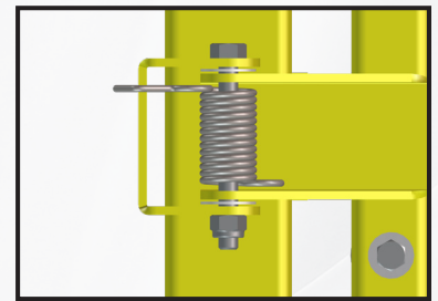
Hinge Detail
