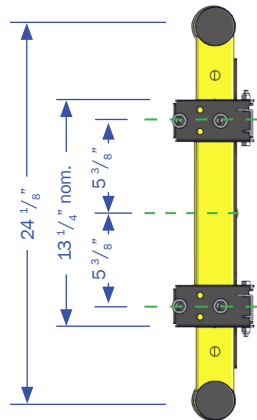
GATE SIDE VIEW
