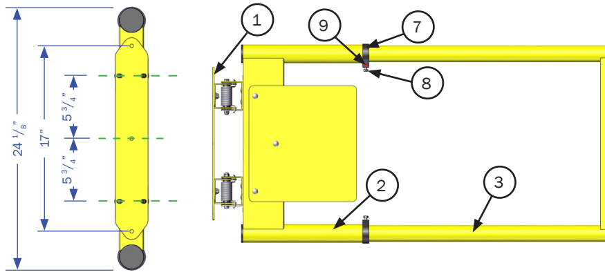
GATE SIDE VIEW
