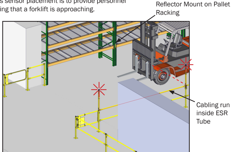
ISO VIEW (ONE ACCESS POINT, TWO LIGHTS)
