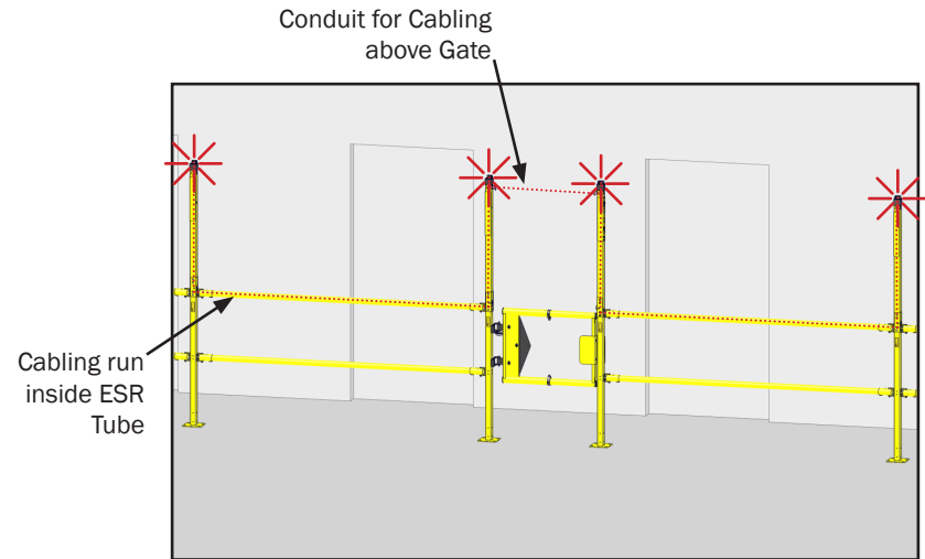
ISO VIEW (ONE ACCESS POINT, FOUR LIGHTS)
