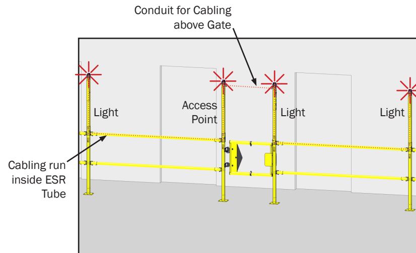
ISO VIEW (ONE ACCESS POINT, FOUR LIGHTS)
