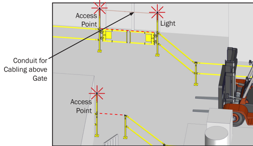
ISO VIEW (TWO ACCESS POINTS, THREE LIGHTS)
