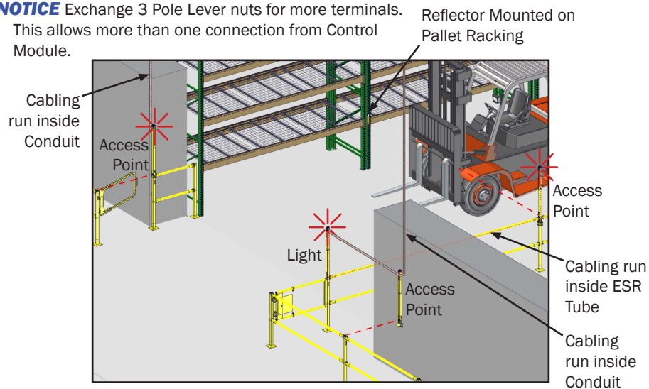
ISO VIEW (THREE ACCESS POINTS, FOUR LIGHTS)
