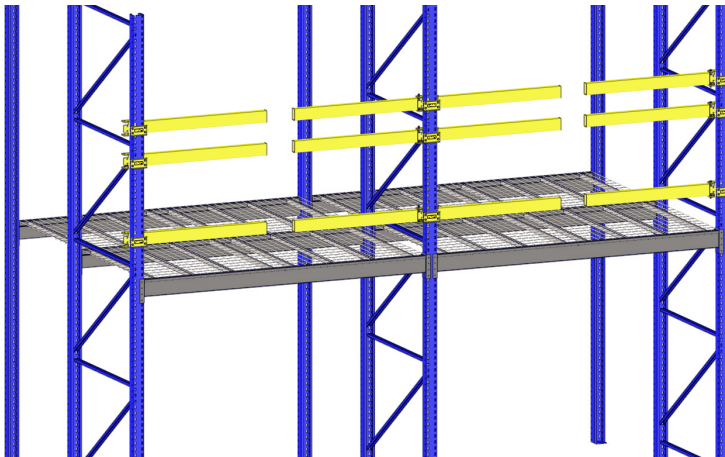
ISO VIEW
